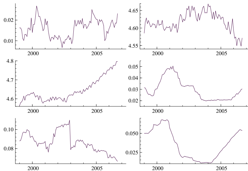
Figure 4. Germany, sub-period 1999-2007, plots of variables (left to right): inflation rate 1 ; index of industrial real wages 1 ; index of industrial production (12 months ahead) 1 ; inter-bank rate 1 ; credit risk premium 2 ; LIBOR US Dollar 3 .
